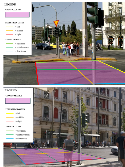
Figure 21 - The use of the custom computer vision pipeline using YOLO and DeepSORT as configured for two specific crossings in the Athens use case area
